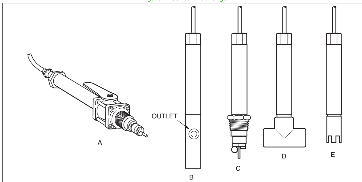
Figure 2. Sensor Mountings
