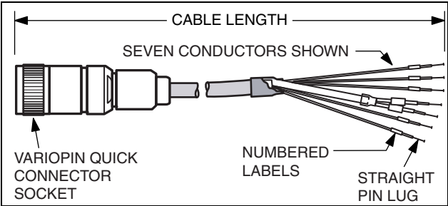
Figure 12. Patch Cord with Variopin Quick Connector Socket
