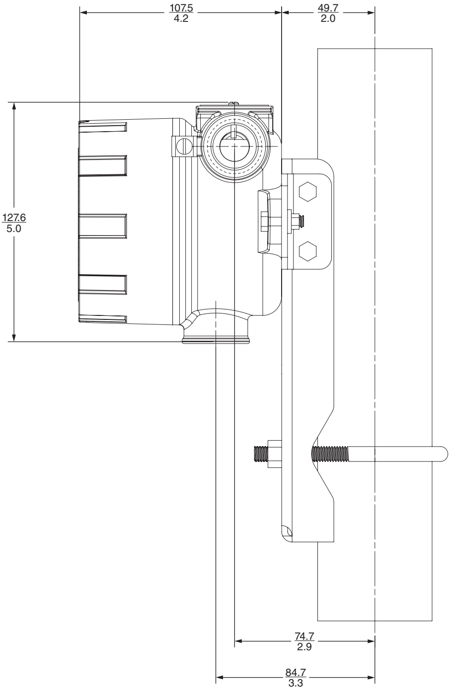
TRANSMITTER WITH HOUSING - PIPE MOUNT - SIDE
