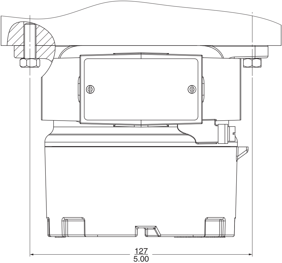
TRANSMITTER WITH HOUSING - WALL MOUNT - TOP
