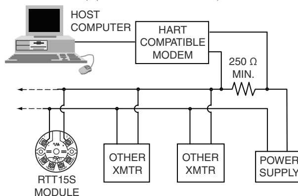
Figure 7. HART Multidrop Block Diagram (Up to Fifteen Transmitters)
