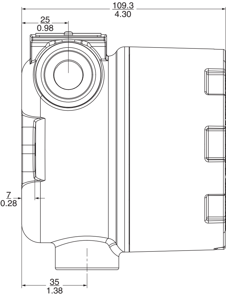
TRANSMITTER WITH HOUSING - SIDE VIEW
