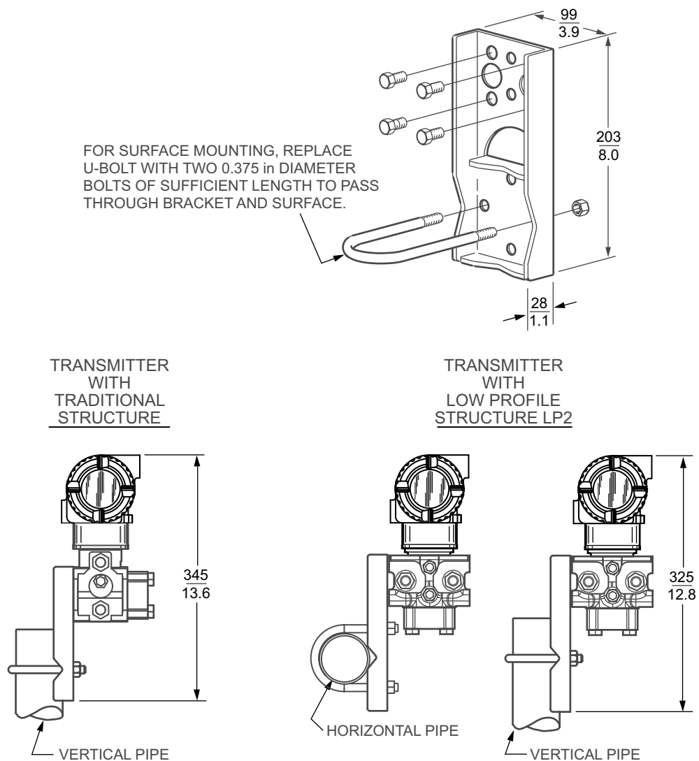
Figure 34 - DP Transmitters with Traditional or LP2 Structure and Options -M1 and -M2 (Standard Style Mounting Bracket)
