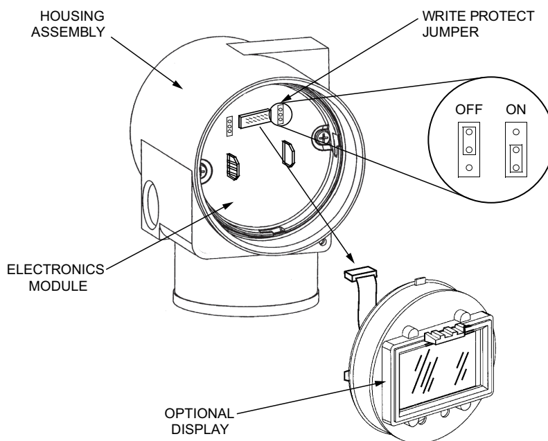
Figure 20 - Write Protect Jumper
